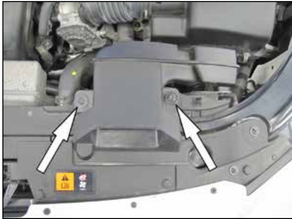
6. Remove the two bolts securing the fresh air intake scoop to the core support.
